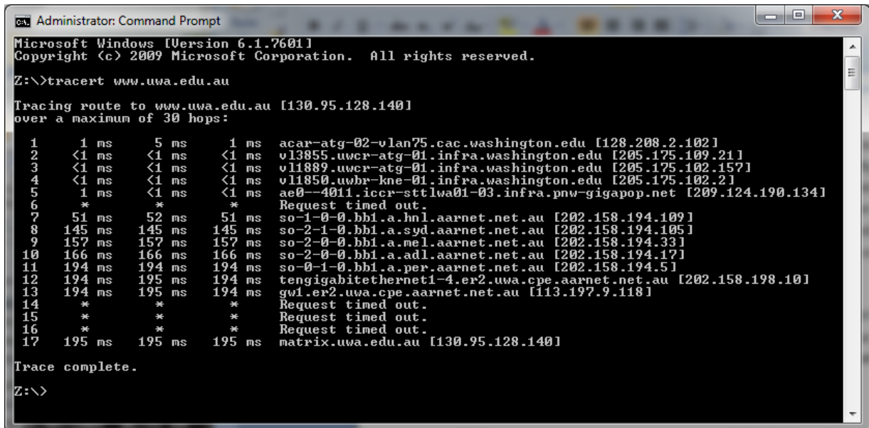
Figure 1: Running traceroute (as tracert on Windows)
